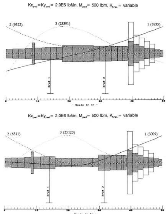
Figure 7. Compressor Computer Models and Undamped Mode Shapes.
