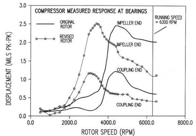
Figure 12. Adjusted Compressor Unbalance Response at Bearings.
