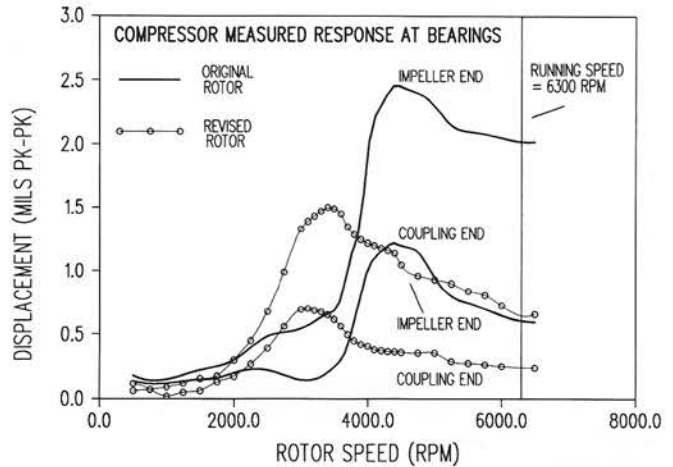
Figure 11. Measured Compressor Unbalance Response at Bearings.
