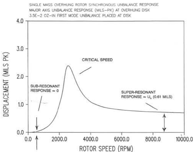
Figure 4. Single-Mass Overhung Rotor Unbalance Response.
