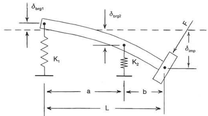
Figure 5. Elastically-Supported Cantilever Beam.
