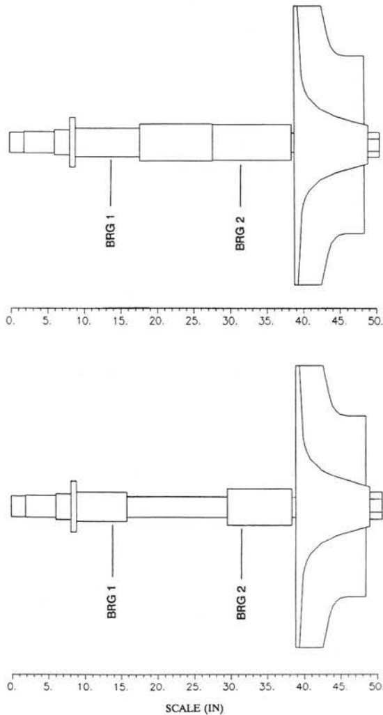
Figure 1. Original and Modified Compressor Rotors.
