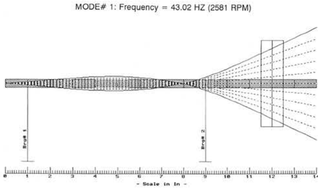
Figure 3. Single-Mass Overhung Rotor First Mode Shape.
