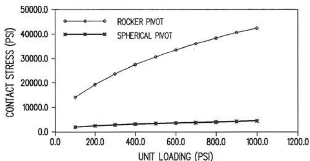
Figure 15. Contact Stresses in Rocker Pivot and Spherical Pivot Bearings.
