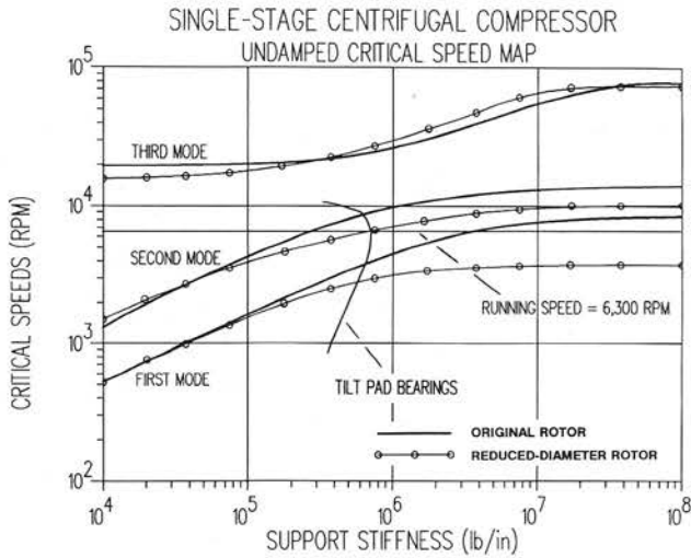
Figure 8. Compressor Undamped Critical Speed Map.
