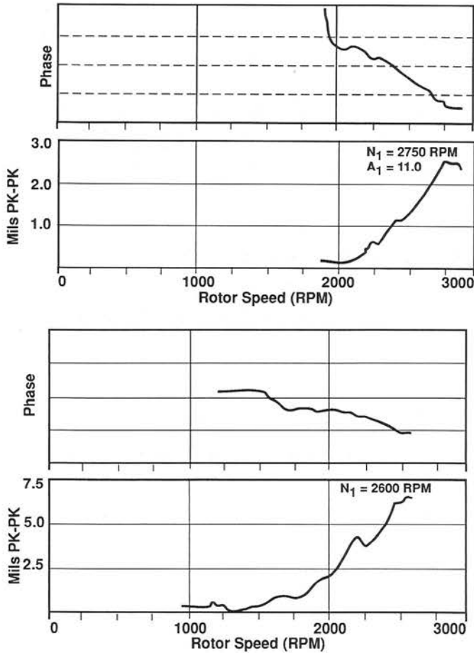
Figure 9. Steam Turbine Field Coast Down, Original Rotor, Tilting Pad Bearings—Coupled.
