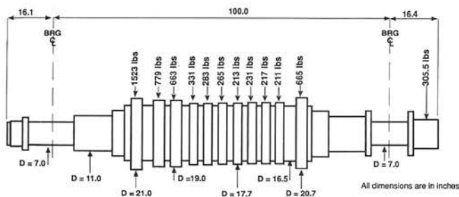
Figure 10. Steam Turbine, Redesigned Rotor, Mass-Elastic Model.
