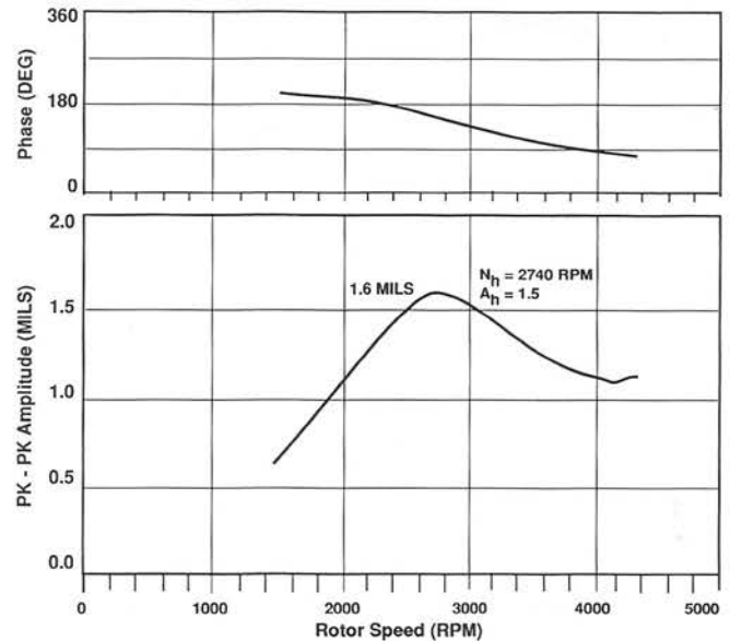
Figure 5. Induction Motor Test Stand Coast Down, Elliptical Sleeve Bearings.
