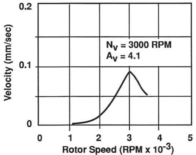
Figure 14. Steam Turbine High Speed Balance Coast Down, Redesigned Rotor, Three Axial Groove Bearings.
