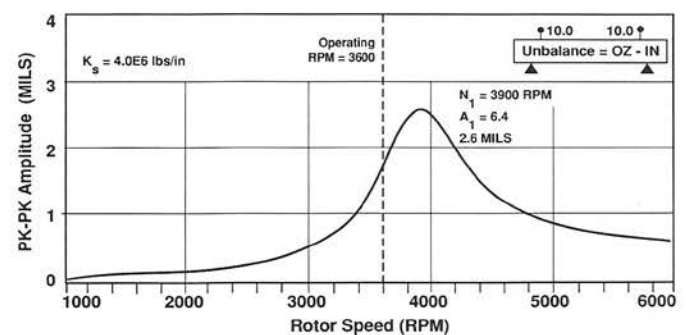
Figure 3. Analytical Speed-Amplitude, Induction Motor, Tilting Pad Bearings.
