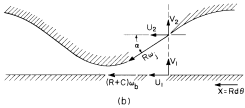
Fig. 4(b). Journal bearing profile unwrapped
