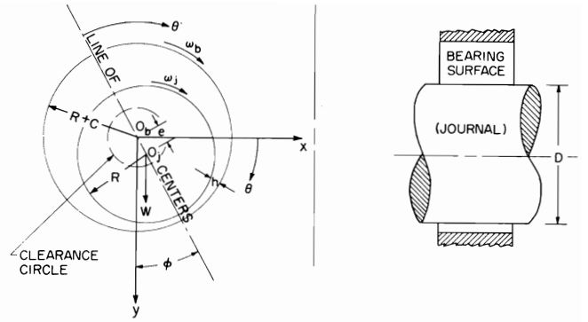
Fig. 1 Short journal bearing configuration
