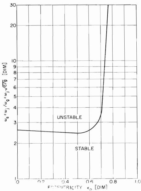
Fig. 14 Stability for the unloaded short journal bearing
