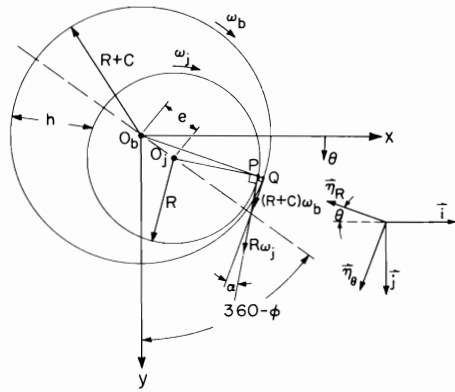
Fig. 5 Journal bearing in fixed Cartesian coordinates
