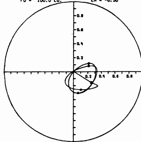
Fig. 15(a) Journal orbit of an unbalanced horizontal rotor having a backward half-frequency rotating load for 5 cycles ( N = 108.3 Hz, W = 22.88 kg, C = 0.0127 cm, L/D = 1/2 , EMU = 0.001 , FO = 444.8 N, EN = -0.5 )
