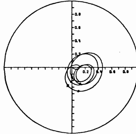
Fig. 10(a) Journal orbit of an unbalanced horizontal rotor at the stability threshold for 5 cycles ( N = 108.3 Hz, W = 22.88 kg, C = 0.0127 cm, L/D = \frac{1}{2} , EMU = 0.2 )
