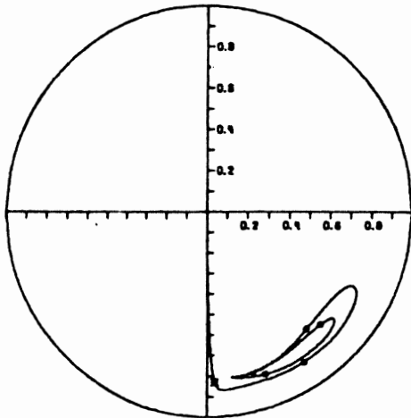
Fig. 6(a) Journal orbit of a balanced horizontal rotor for 5 cycles ( N = 108.3 Hz, W = 816.48 kg, C = 0.0127 cm, L/D = \frac{1}{2} )
