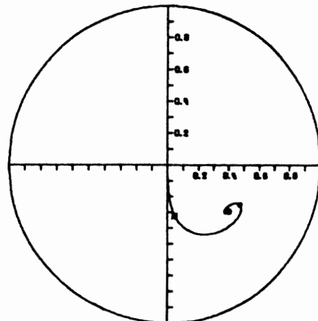
Fig. 7 Journal orbit of a horizontal balanced rotor with constant load for 5 cycles ( N = 108.3 Hz, W = 22.68 kg, C = 0.0127 cm, L/D = \frac{1}{2} , FOCY = -867.26 N)
