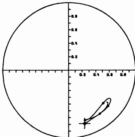
Fig. 6(b) Journal orbit of a balanced horizontal rotor for 5-10 cycles ( N = 108.3 Hz, W = 816.48 kg, C = 0.0127 cm, L/D = \frac{1}{2} )
