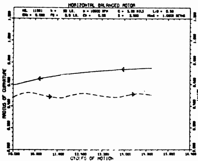
Fig. 4(b) Radius of curvature and whirl versus cycles of motion for cycles 10-18 ( N = 175 Hz)
