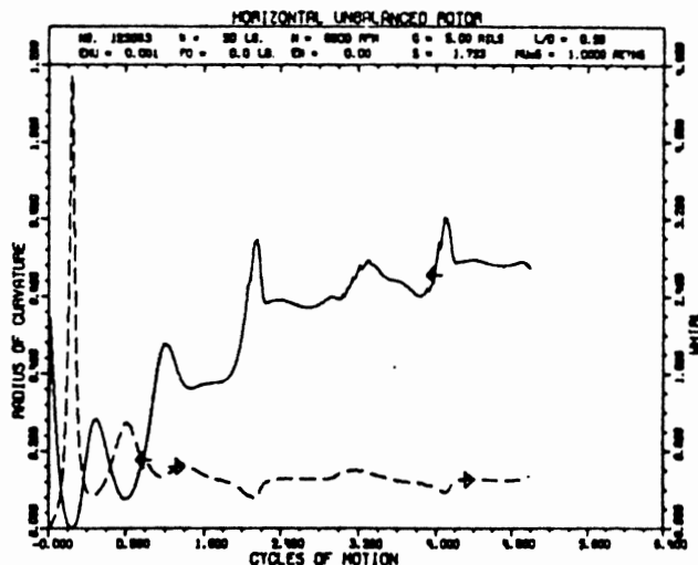
Fig. 16(b) Radius of curvature and whirl versus cycles of motion ( FHY = 444.8 N, ENY = 0.5 )
