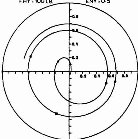
Fig. 16(a) Journal orbit of an unbalanced horizontal rotor having unidirectional harmonic loading for 5 cycles ( N = 108.3 Hz, W = 22.68 kg, C = 0.0127 cm, L/D = \frac{1}{2} , EMU = 0.001 , FHY = 444.8 N, ENY = 0.5 )
