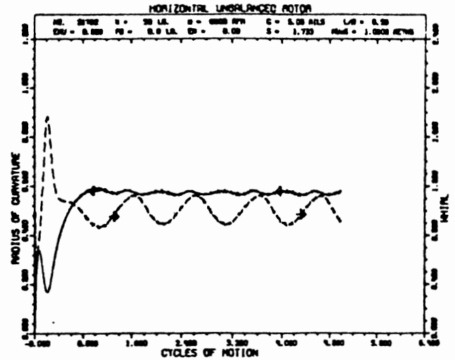
Fig. 11(c) Radius of curvature and whirl versus cycles of motion ( N = 108.3 Hz)
