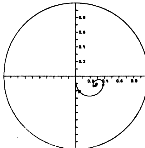
Fig. 2(a) Journal orbit of a balanced horizontal rotor ( N = 66.67 Hz., W = 22.68 kg, C = 0.0127 cm, L/D = \frac{1}{2} )
