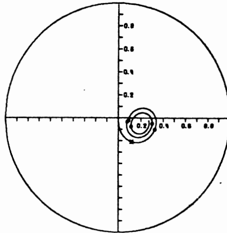
Fig. 3(a) Journal orbit of a balanced horizontal rotor ( N = 108.3 Hz, W = 22.68 kg, C = 0.0127 cm, L/D = 1/2 )
