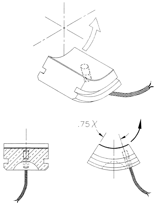
Figure 6. Self Aligning Pad Temperature Sensor Location.
