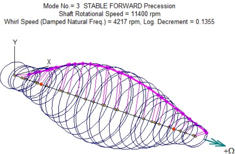
Figure 29 Stability Analysis of the New Rotor Design with the Original Five Pad LOP Bearings
