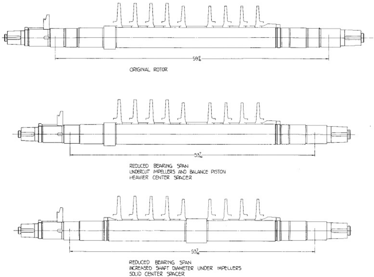
Figure 4 Redesign of the Compressor Rotor. From Smith (13)
