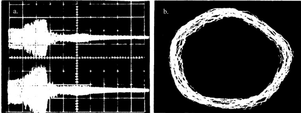
Figure 2. (a) Time-lapse and (b) orbit of the instability onset. From Smith (13).
