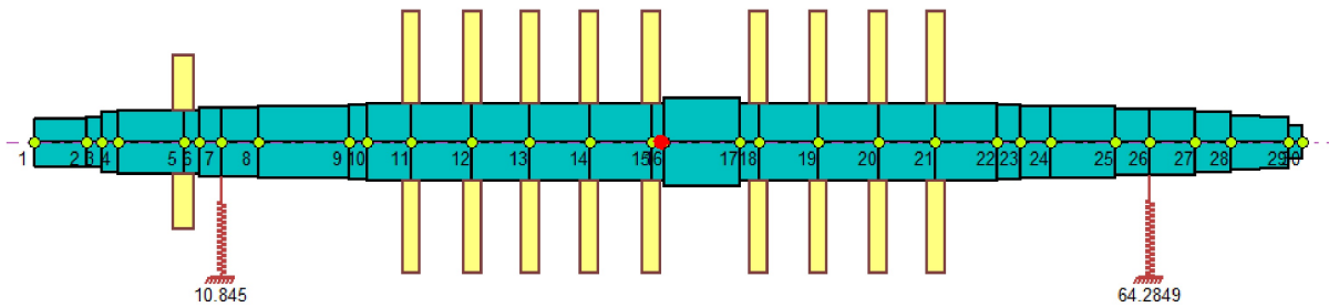
Figure 27 Reduced Bearing Span Shaft Model
