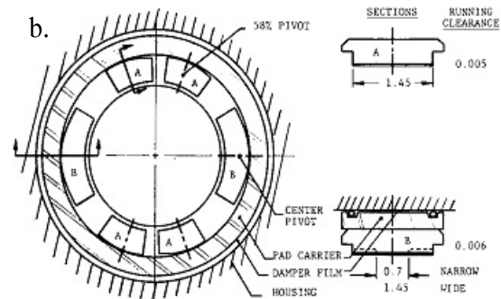
Figure 3(b) Squeeze Film Damper Design Smith (13)
