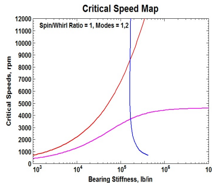
Figure 6 Compressor Critical Speed Map
