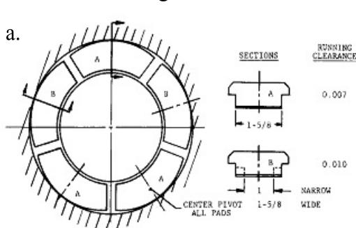
Figure 3(a) Asymmetric Tilt Pad Bearing Smith(13)
